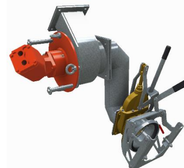
TURBO-MASTER 8-6
